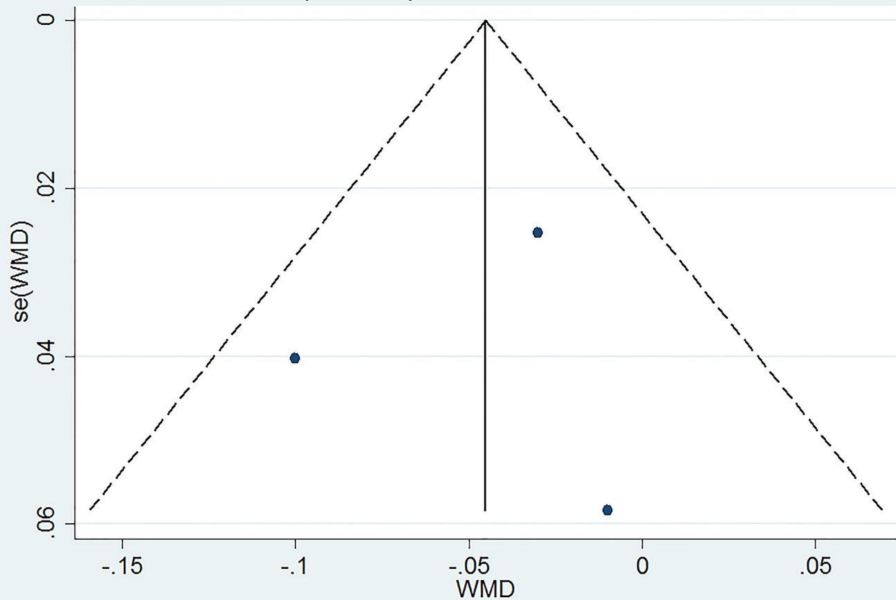
Funnel plot with pseudo 95% confidence limits
