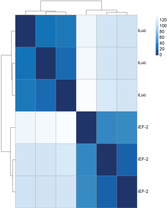
B. Heatmap of sample-to-sample distances using rlog-transformed counts
