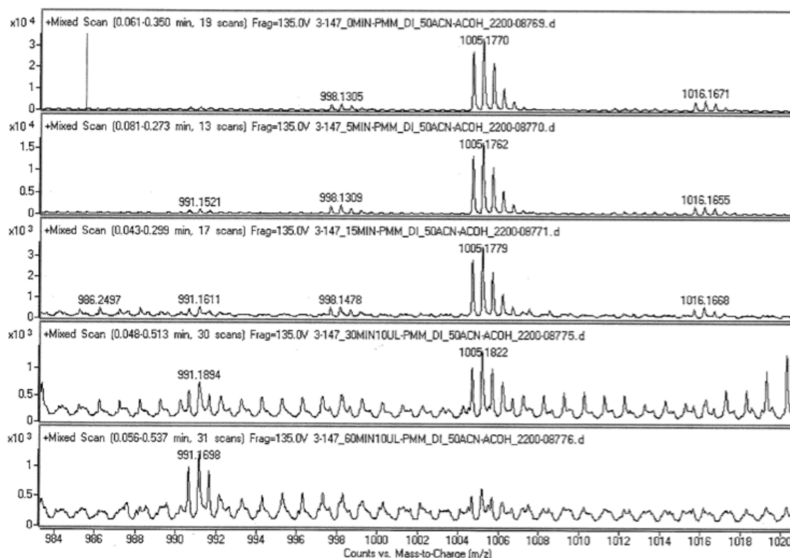
Figure S10: Evaluation of RCM on peptide 23 as a function of time ( t = 0 to 60 min). The indicated mass corresponding to starting material 23 (1005.1770) and product 29 (991.1698) is observed as the [M+2H]^{2+} ion as measured by LC/MS TOF
