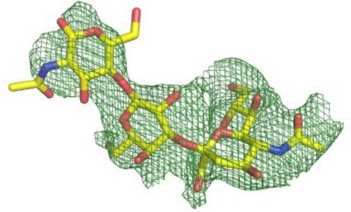
Omit (Fo-Fc) map
