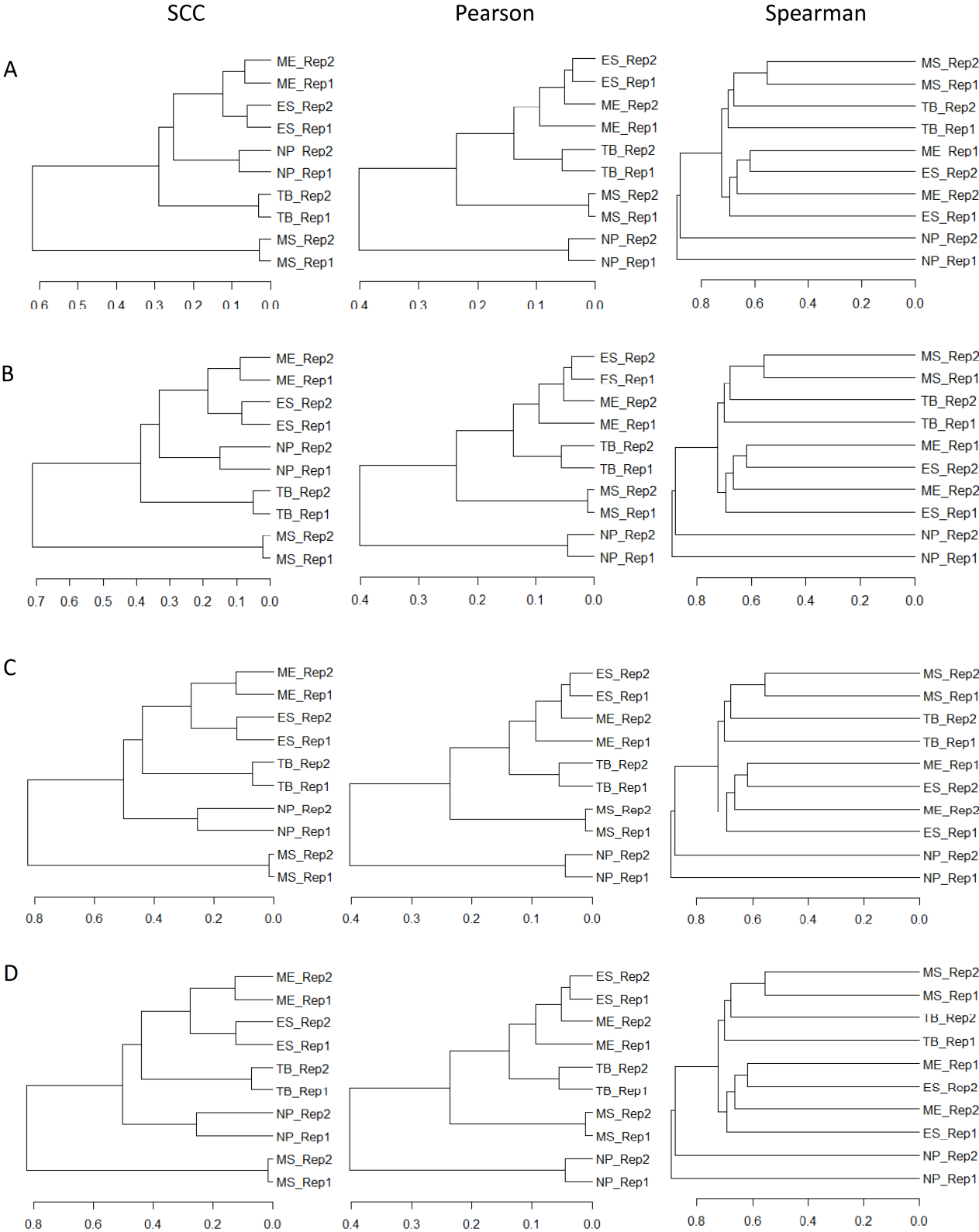
Supplemental Figure S5. Relationship between the ten samples in the human H1 ES cell lineage estimated using interactions at different distance ranges, (A) 0-4M, (B) 0-6M, (C) 0-8M, and (D) 0-10M by SCC (Left), Pearson (Middle) and Spearman (Right).
