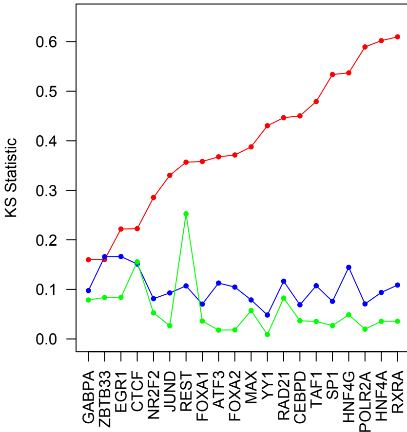
Supplemental_Fig_S11. Dots represent KS-statistic of enrichment for proximal binding of each DAP to liver (red), skin (blue) and cortex (green) -specific genes in child liver tissue.
