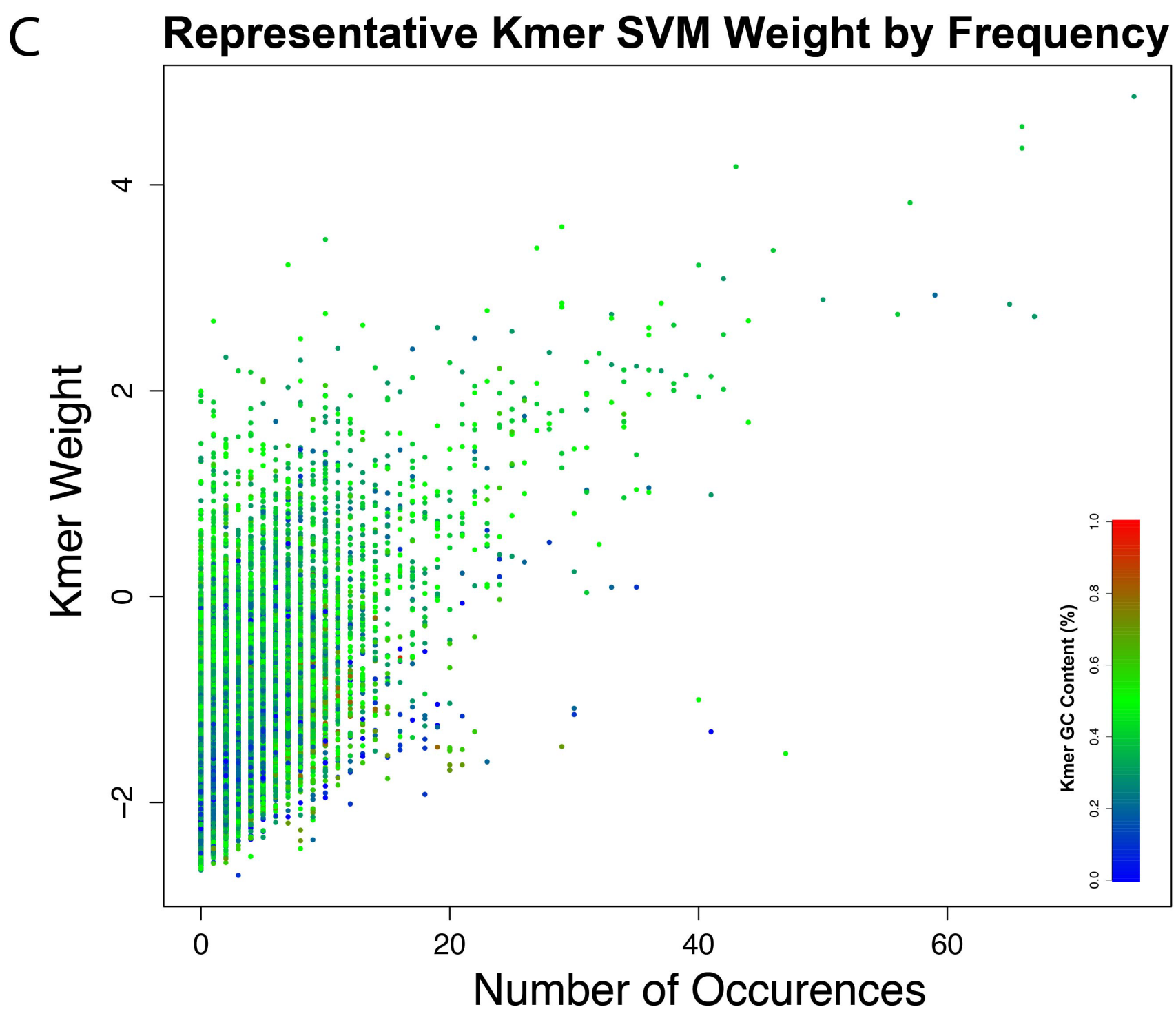
Supplemental_Fig_S16. (A) ROC curve AUC values for SVMs trained on each DAP. (B) Precision-recall curve AUC vales for SVMs trained on each DAP. Representative plot for SVM models in ATF3. Plots the frequency of each 10mer in ATF3 binding sites against its SVM weight. Color of each point reflects the GC content of the 10-mer.
