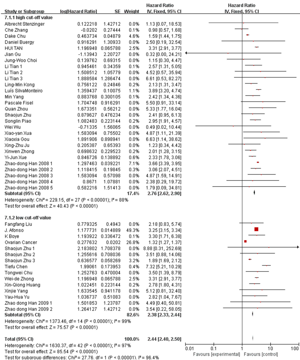
Supplementary Figure 2: Subgroup analysis based on the EMMPRIN positive expression determination.
