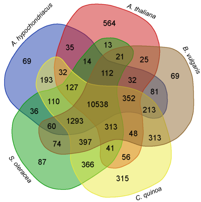
Supplementary information, Figure S6 Venn diagram showing the overlap of orthologous groups among quinoa and 4 other plant species.
