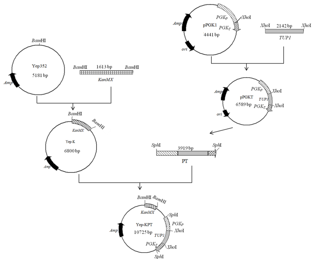
Fig. S1 Construction process of the plasmid Yep-KPT.
