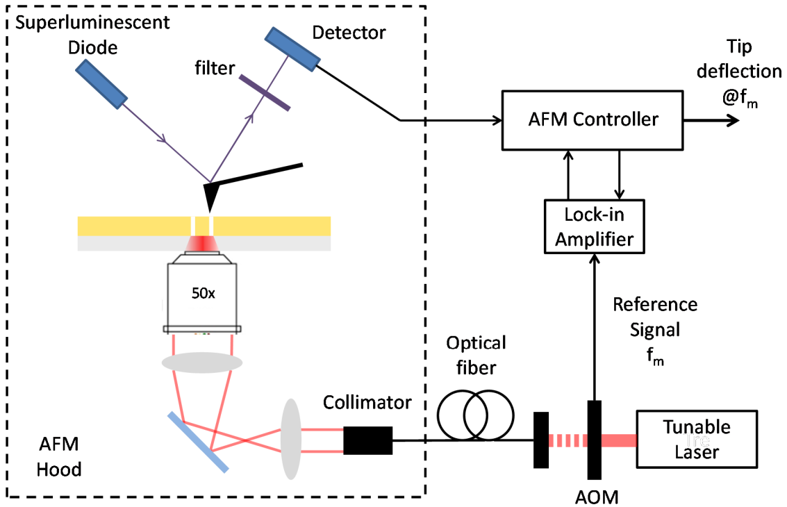
Supplementary Fig. 1| Experimental setup for optical force measurement. AOM represents acoustic optical modulator. f_m is modulation frequency of the AOM. The AFM hood indicates the temperature and vibration control chamber.
