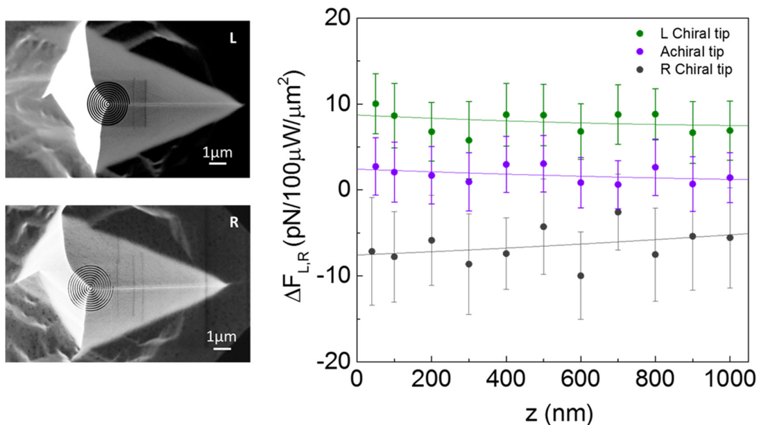
Supplementary Fig. 7 | Enantioselective optical forces measured with tips patterned with L- and R- chiral spirals, and an achiral tip as a function of tip-aperture separation ( z ). The solid lines are polynomial fitting to the data. The SEM images on the left are top-views of the L- and R- chiral spiral patterned tips.
