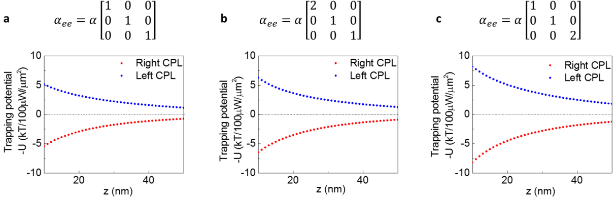
Supplementary Fig. 11| Calculated trapping potentials as a function of tip-aperture separation when considering the anisotropy of the tip. a, The tip is considered as an isotropic sphere; b, the tip is considered as an anisotropic sphere with anisotropy along the x direction; and c, the tip is anisotropic along the z direction.
