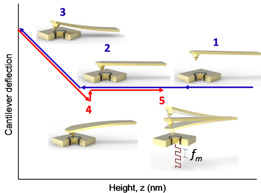
Supplementary Fig. 2| A schematic illustration of the measurement used in this study. A force-distance curve is first performed to locate the exact tip-aperture separation. When the tip retracts to a certain height, z , a gated CW laser source is turned on, with a repetition rate that matches the fundamental mechanical resonance of the cantilever.
