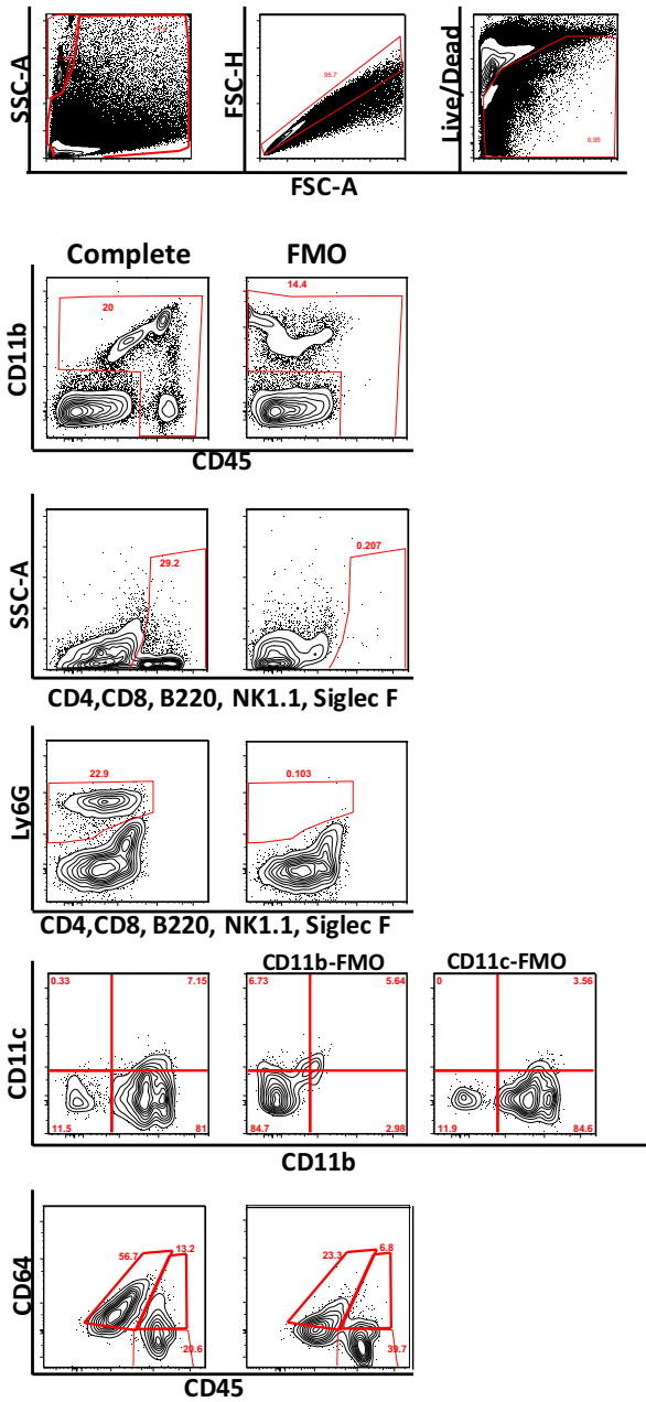
Figure S1: Fluorescence minus one analysis of fluorochrome panel: Mice underwent TBI and the brains were harvested and processed as previously described. The single cell suspension was then divided equally and fluorescently labelled with the antibody panel (see Table 1). Each panel had one fluorochrome missing to determine the proper placement of the gates for our flow cytometric analysis.
