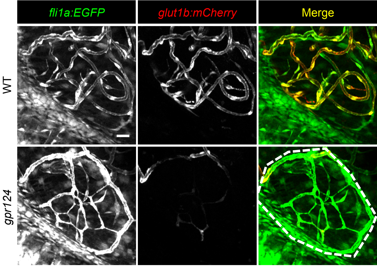
Supplemental Figure 1. gpr124 mutants form abnormal vessels on the brain surface at 6 dpf. Shown here is a high magnification of the images shown in Figure 3D. Scale bar in top left image is 10 \mu m for all images.
