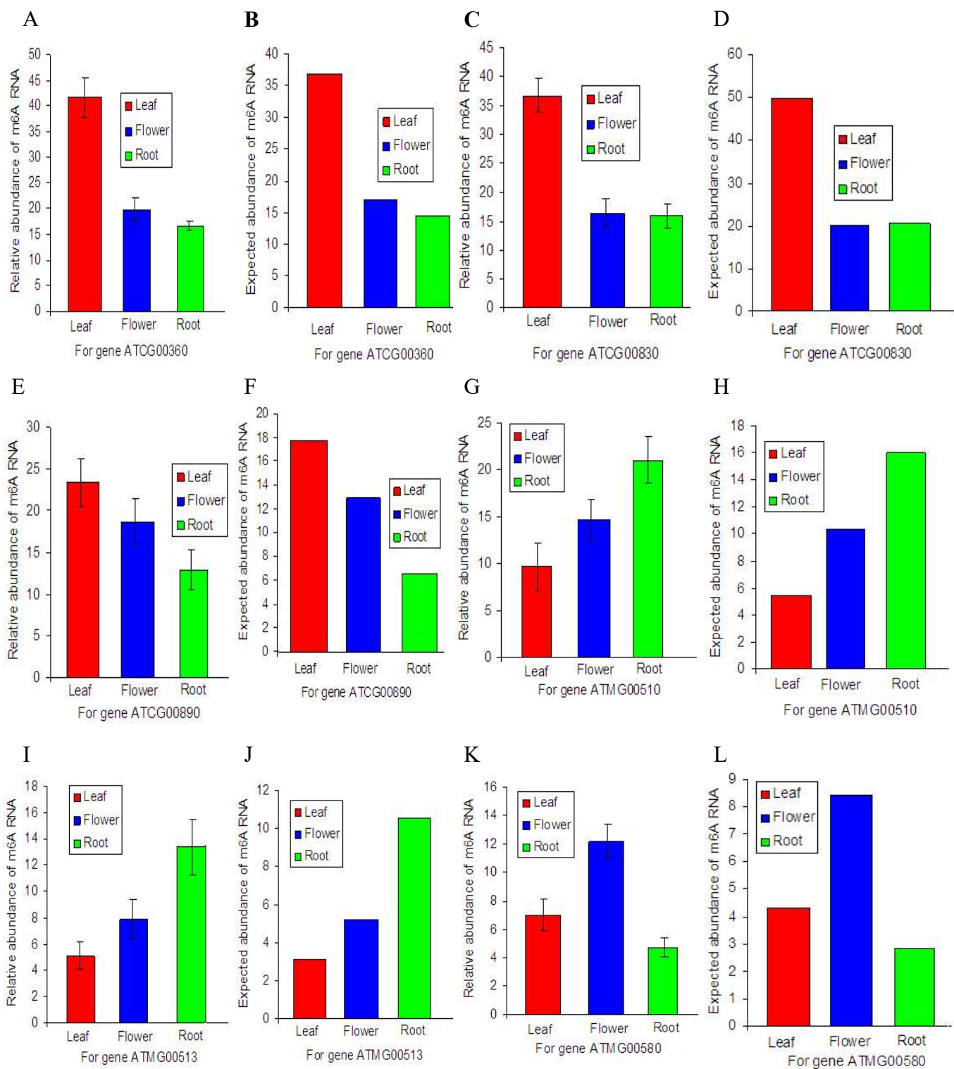
S2 Fig. The relative abundance (RA) of m 6 A RNA deduced from qRT-PCR and the expected abundance (EA) of m 6 A RNA deduced from the m 6 A-seq data set.
