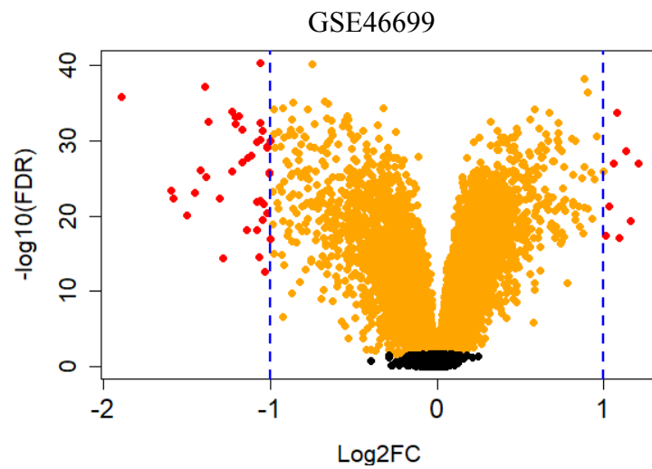
Supp. Figure 1. The volcano plots of the expression of four ccRCC data sets.
