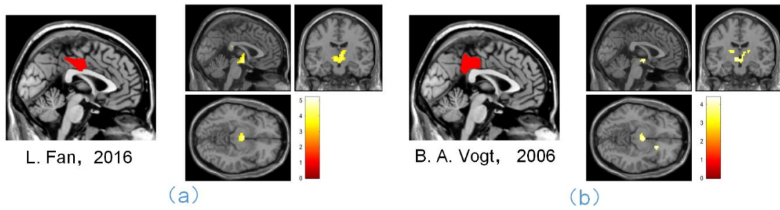
Supplementary Figure 1 the brain regions which functional connectivity with dorsal posterior cingulate cortex showed significant association with trait urgency ( P_{\text{FWE}} = 0.05 , family-wise error (FWE) correction). (a) Seed region was defined from the Human Brainnetome Atlas (bilateral CG-6 region, L. Fan, 2016). (b) Seed region was anatomically defined by bilateral dorsal posterior cingulate cortex (B. A. Vogt, 2006).
