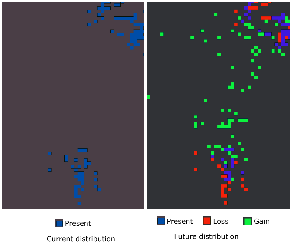
S1 Fig. An example to show predicted gain and loss areas in the future distribution of one species.
