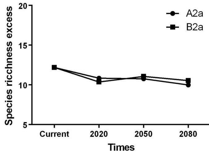
S7 Fig. Species richness excess inside relative to outside PAs using binary distribution (assuming no dispersal).
