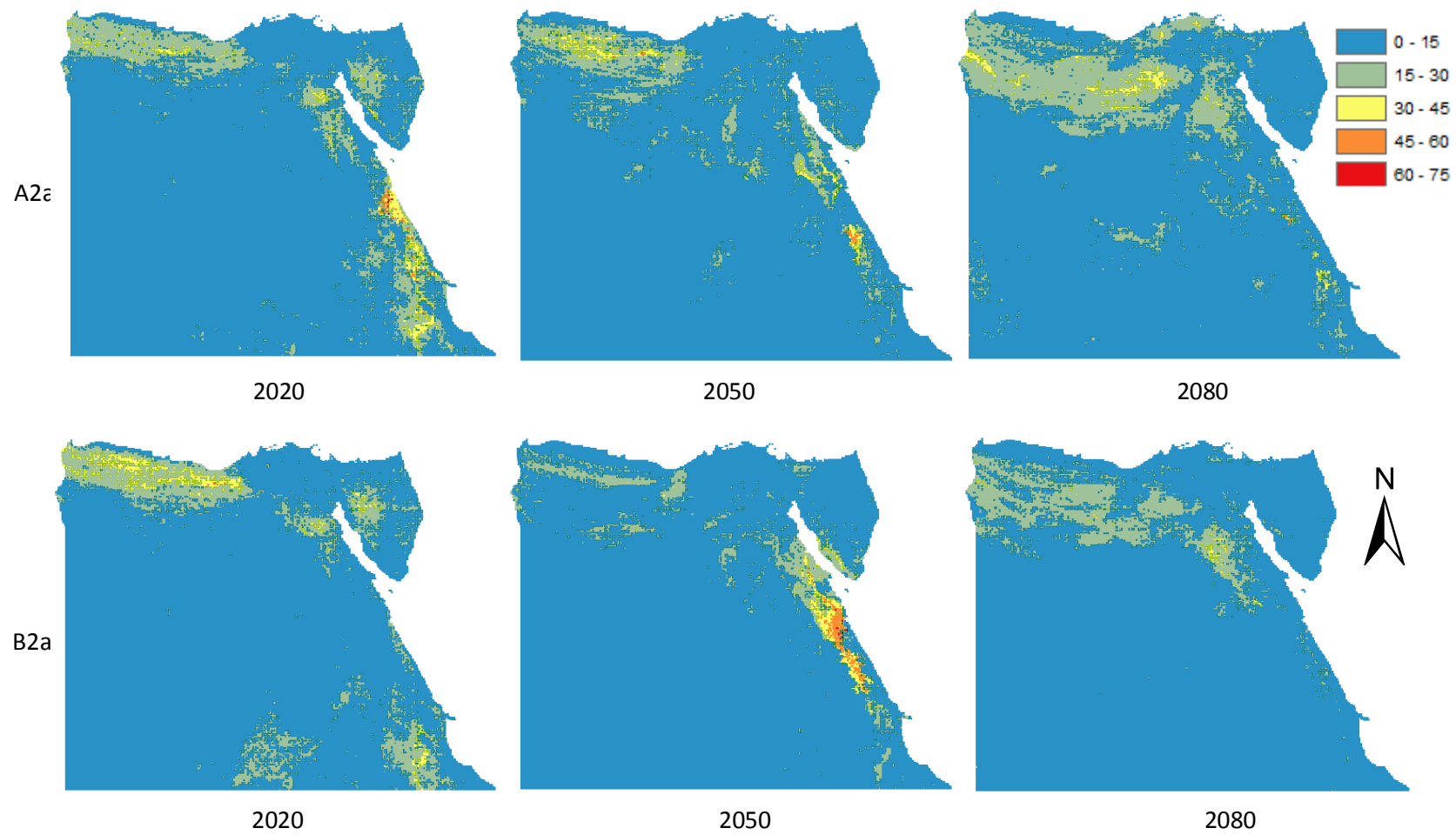
S8 Fig. Spatial pattern of the number of species gained under climate change in the future (assuming unlimited dispersal). Colours indicate few (blue) to many (red) species gained.
