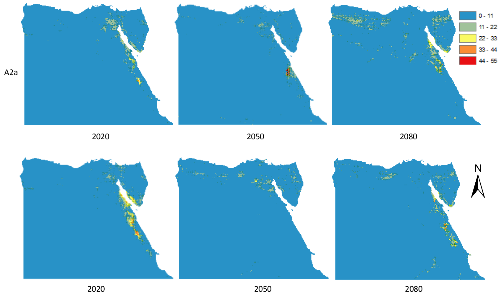
S9 Fig. Spatial pattern of the number of species lost under climate change in the future (assuming unlimited dispersal). Colours indicate few (blue) to many (red) species lost.
