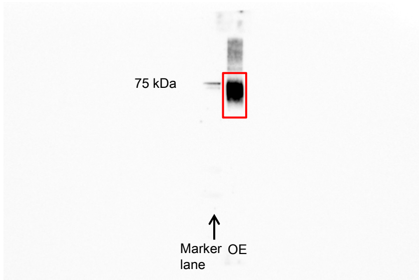
SLCO2A1 overexpression in HEK
