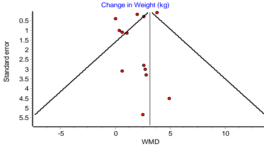
Figure S7 Funnel plot for weight
