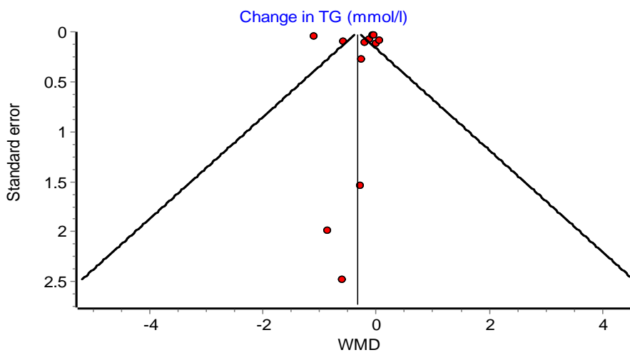
Figure S6 Funnel plot for TGs
