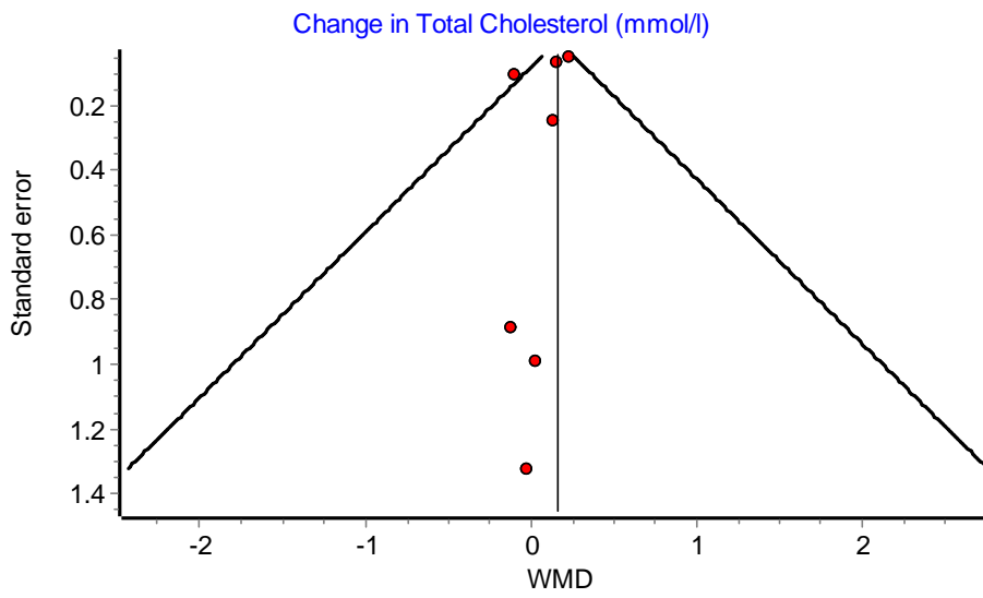
Figure S3 Funnel plot for total cholesterol
