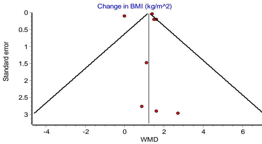
Figure S8 Funnel plot for BMI
