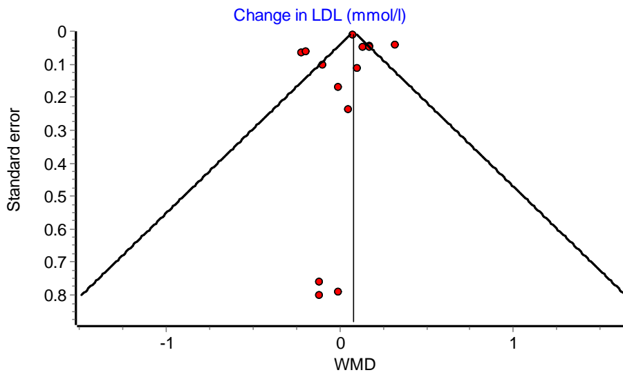
Figure S4 Funnel plot for LDL
