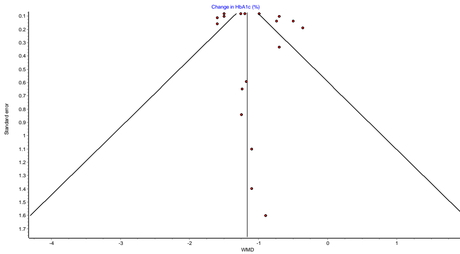
Figure S2 Funnel lot for HbA1c
