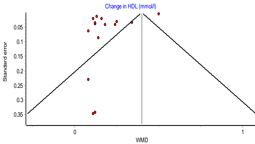
Figure S5 Funnel plot for HDL
