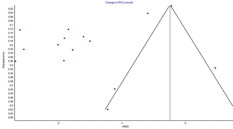
Figure S1 Funnel plot for FPG
