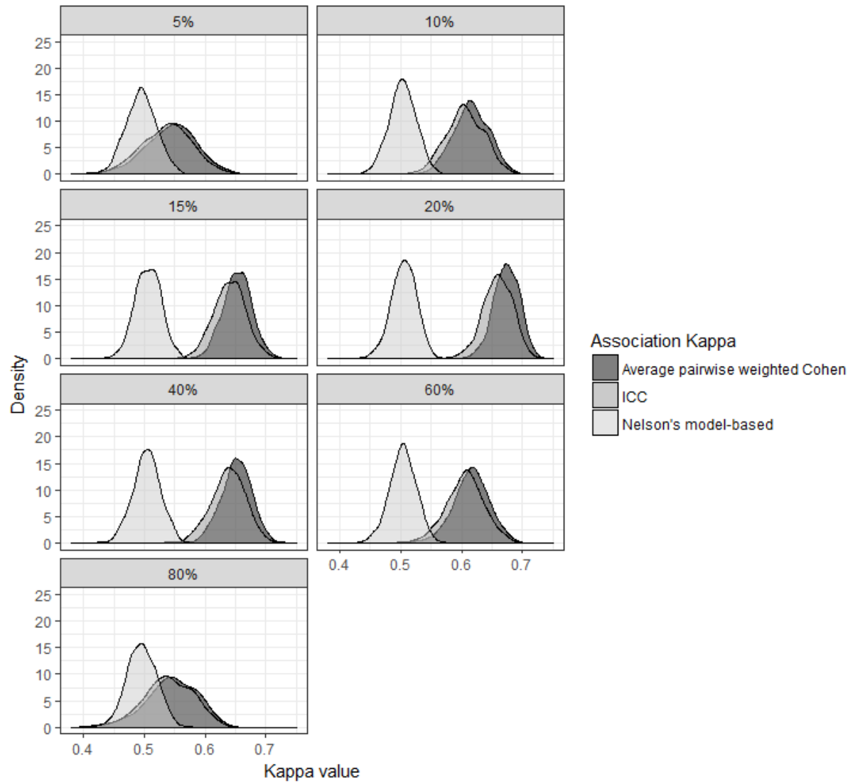
Supplementary Figure 1b. Density of Simulated Measured Association Values by Prevalence in Category 1
