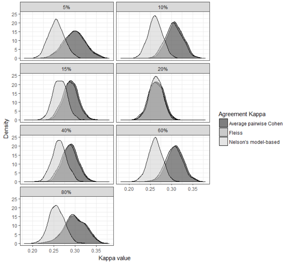
Supplementary Figure 1a. Density of Simulated Measured Agreement Values by Prevalence in Category 1
