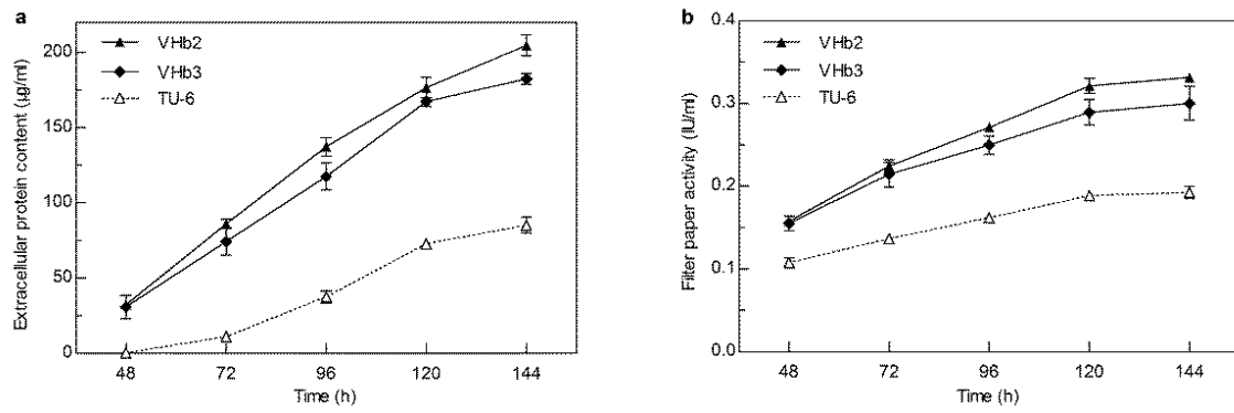
Figure S2 Time course determination of the extracellular protein concentration (a) and FPase activity (b) in the Vhb-expressing strains Vhb2 and Vhb3 in cellulase-inducing medium under oxygen-limiting conditions. Vhb2 (filled triangle) and Vhb3 (filled diamond) are shown as black solid lines and TU-6 (hollow triangle) is shown as dashed lines. Data represented are the means of three independent cultures
