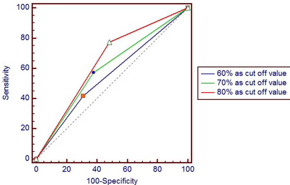
Supplementary Figure 1: Receiver operating characteristic curve to compare the AUCs with 60%, 70% and 80% positive immune cell infiltrates as cut-off values. Blue line: 60% as cut-off value, AUC= 0.553; Green line: 70% as cut-off value, AUC=0.596; Red line: 80% as cut-off value, AUC=0.646.
