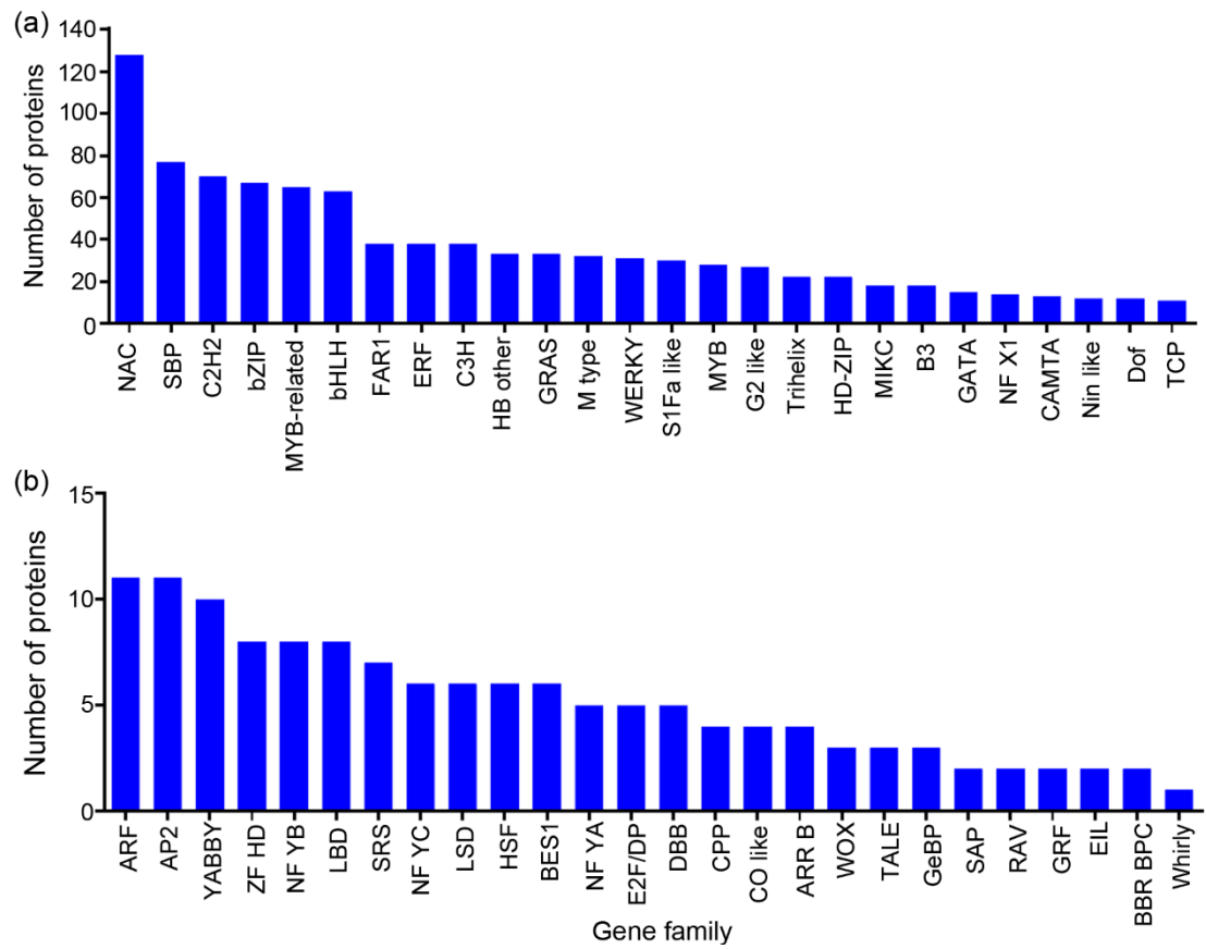
Fig. S1. Gene family of membrane-bound transcription factors in the 14 plant species.
