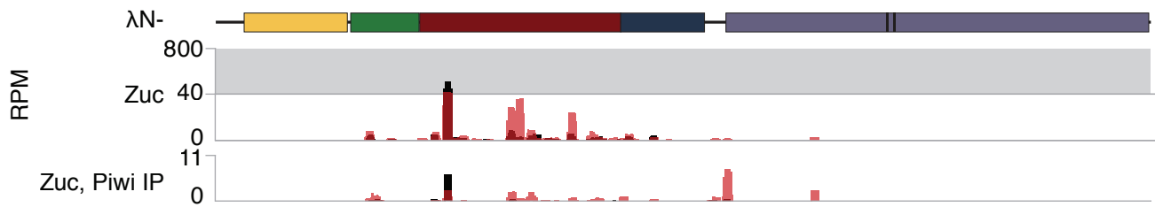
Supplemental Figure 1. Upon Zuc tethering reporter derived sequences that are 25-28nt in length (black) map along the whole body of the reporter, whereas 22-23nt reads (red) map predominantly at the 5' region of the reporter transcript. Shown are profiles for reads specifically mapping to the reporter, normalized to all reads mapping to the DM3.
