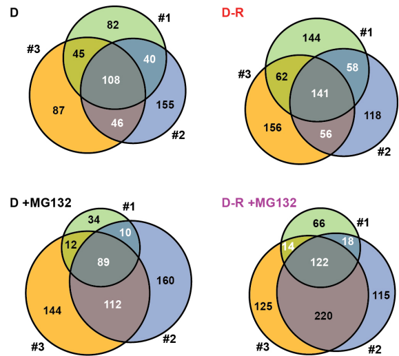
Supplemental Figure 2. Venn Diagrams Comparing the MS Datasets from Three Biological Replicates Obtained from Dark Grown Arabidopsis Seedlings Before (D) and After Red-Light Irradiation (D-R) and MG132 Exposure. The number of proteins in each sector is indicated.
