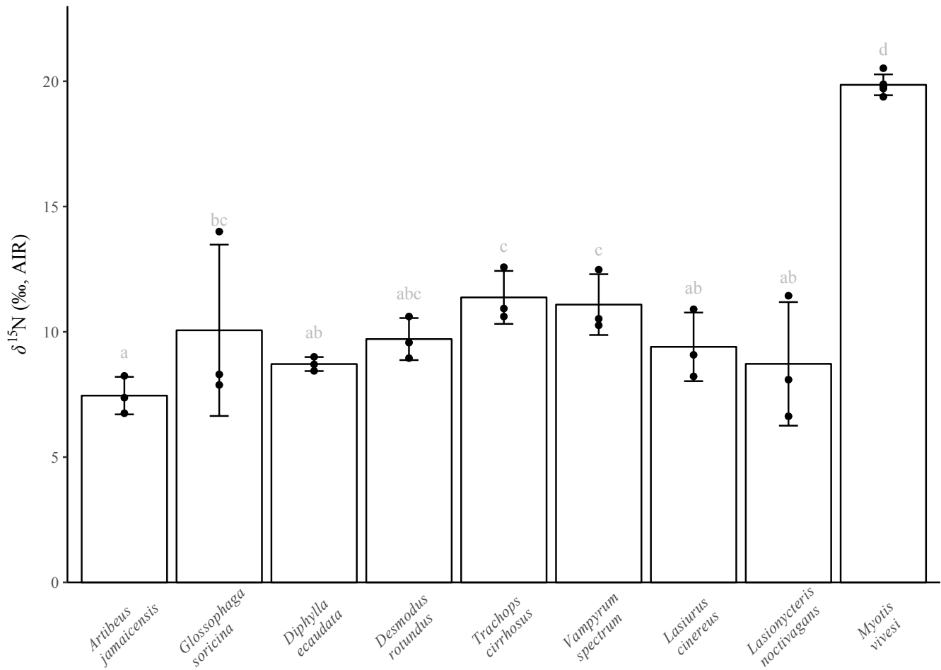
Sup. Fig. 1 \delta^{15}\text{N} values of bulk hair samples. Letters indicate species-level differences in \delta^{15}\text{N} values determined by Tukey's test of mean comparison.
