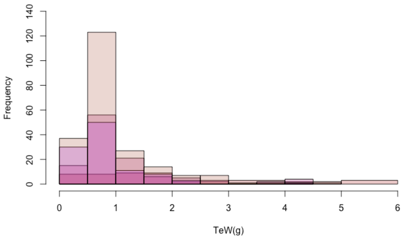
Histogram for TeW in different genotype classes
