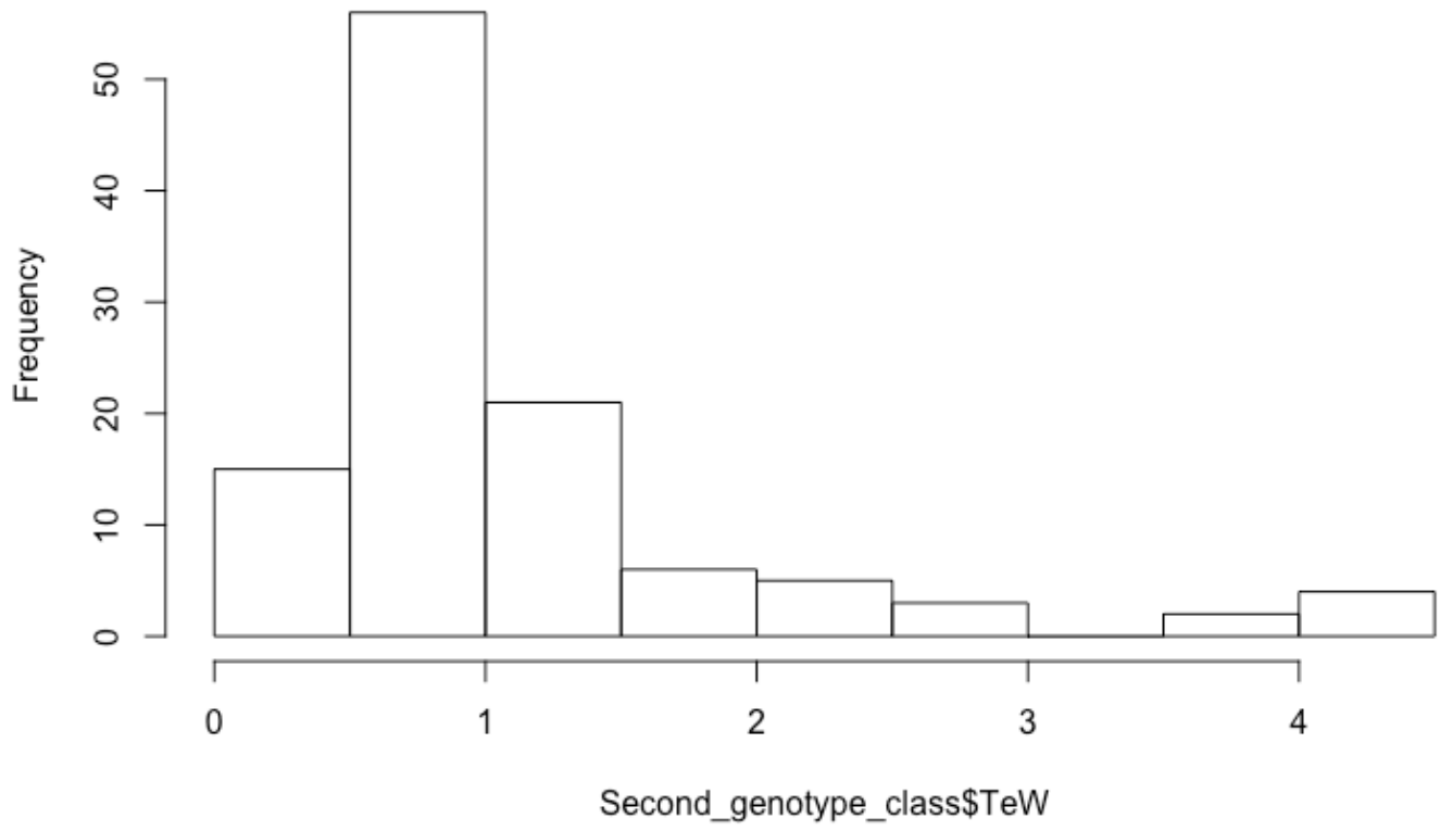
Histogram of Second_genotype_class$TeW
