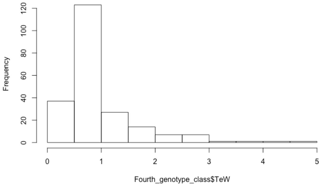
Histogram of Fourth_genotype_class$TeW
