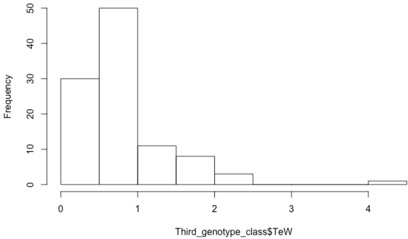
Histogram of Third_genotype_class$TeW
