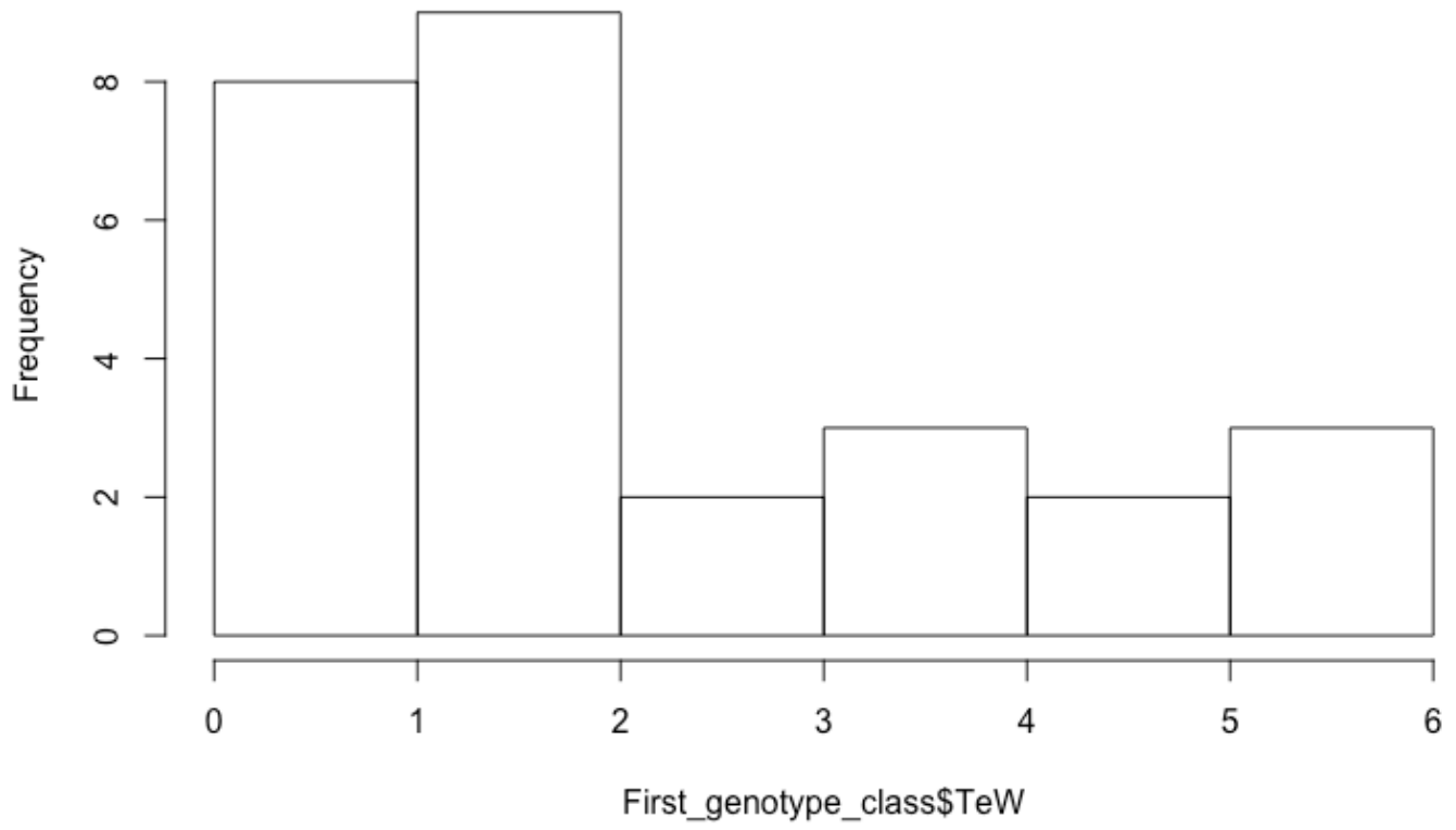
Histogram of First_genotype_class$TeW
