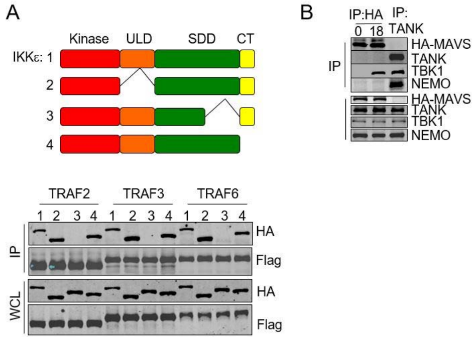
Fig S3. TBK1/IKKε are recruited to MAVS via the pre-associated TRAFs-TBK1/IKKε.
