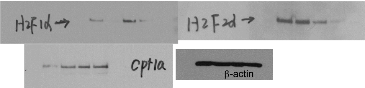
Figure 5 blots:
