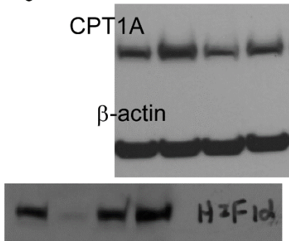
Figure 7 blots:
