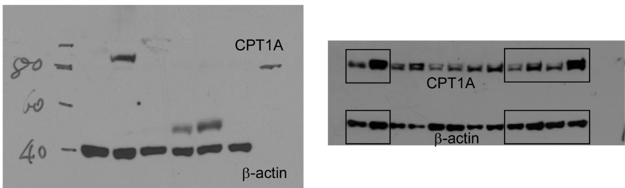
Figure 7 blots:
