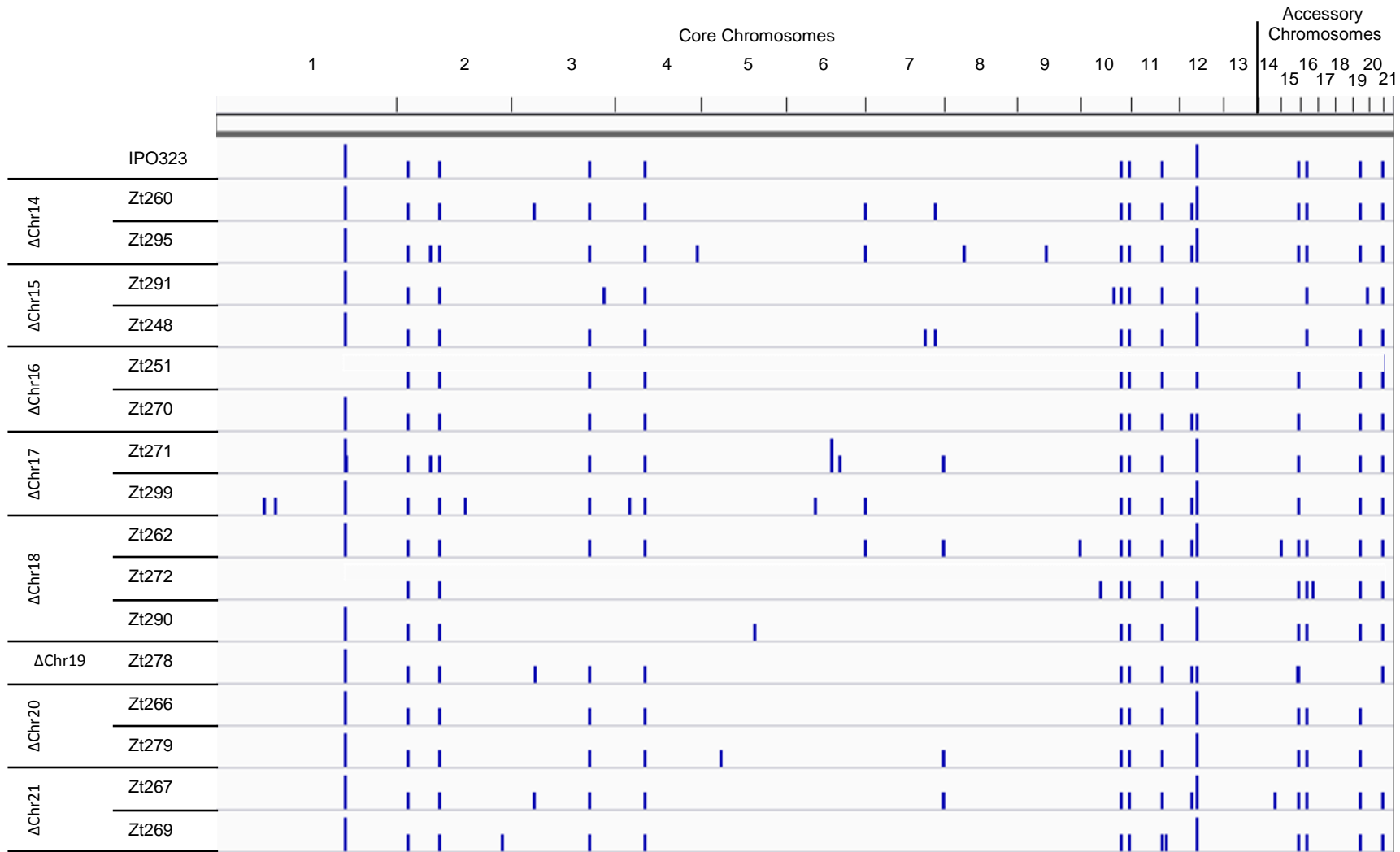
FIG S4 Illustration of the location of all single nucleotide polymorphisms (SNPs) and indels identified in all sequenced strains. Genome-wide distribution of SNPs across the thirteen core and eight accessory chromosomes of the reference strain IPO323.
