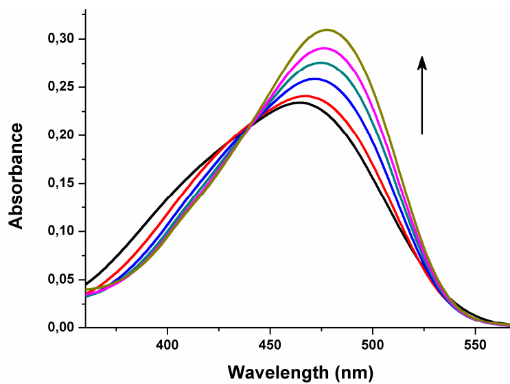
Figure S1. Absorption spectra of 10 μM methyl orange in the absence and presence of increasing HSA concentrations (5, 10, 15, 20, and 30 μM) in PBS.
