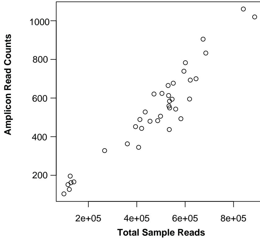
Read Counts Versus Total Reads for a Typical Amplicon
