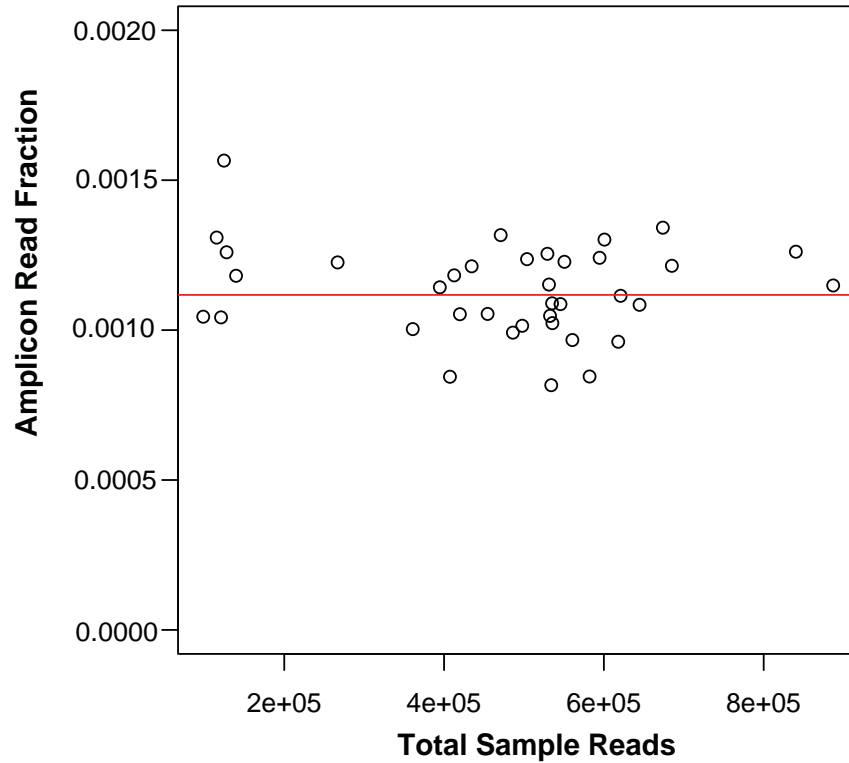
Read Counts Normalized by Total Reads for a Typical Amplicon
