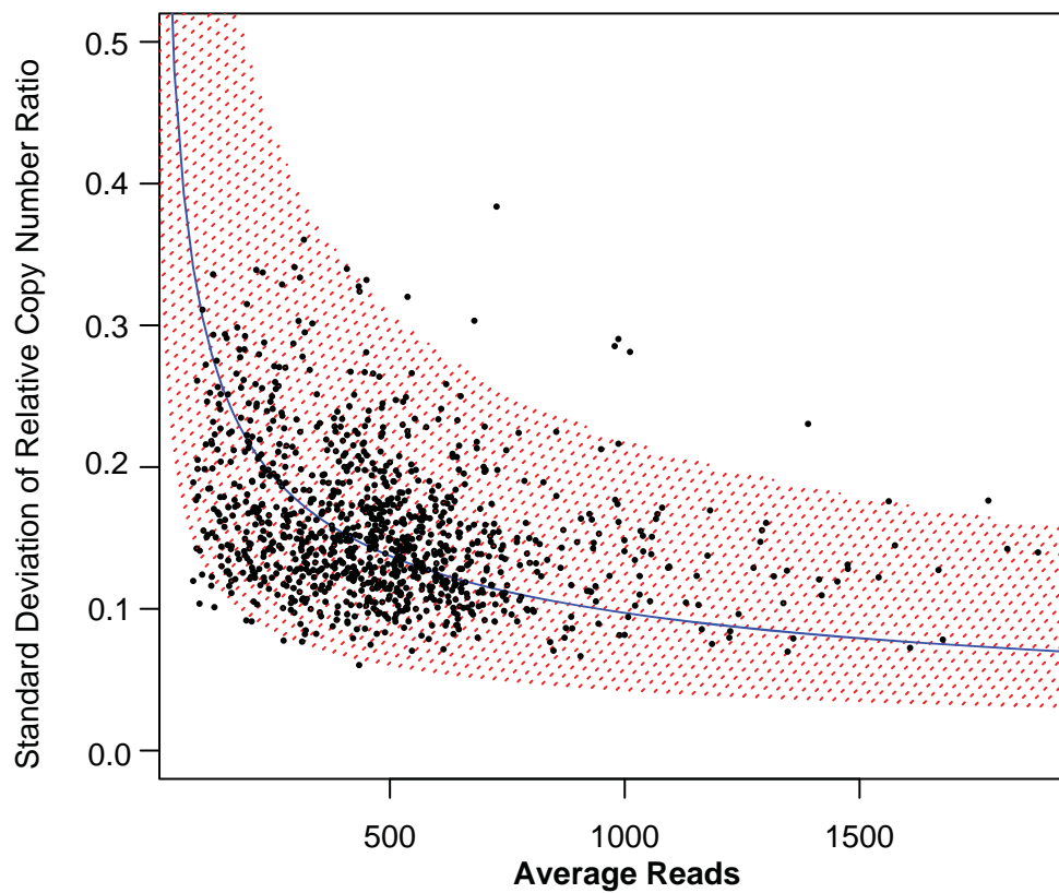
Probe Variance in Matched Tumors
