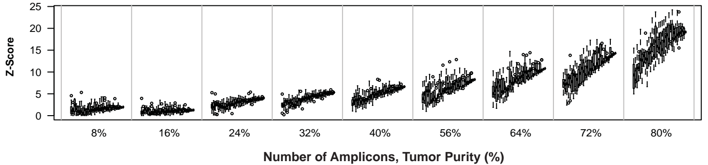
RB1 Significance for Increasing Number of Amplicons and Tumor Purity
