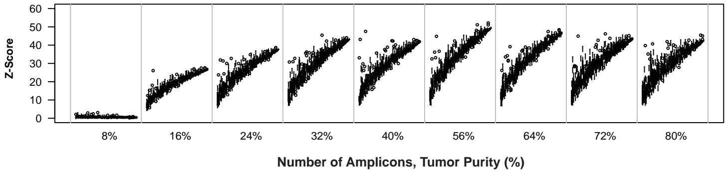
ERBB2 Significance For Increasing Number of Amplicons and Tumor Purity
