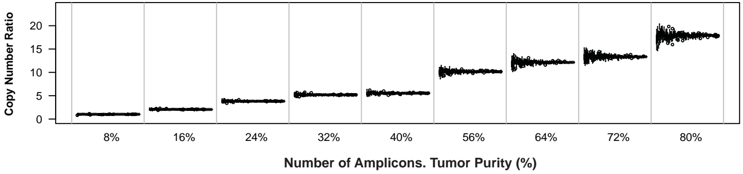
ERBB2 Fold Change Estimate For Increasing Number of Amplicons and Tumor Purity
