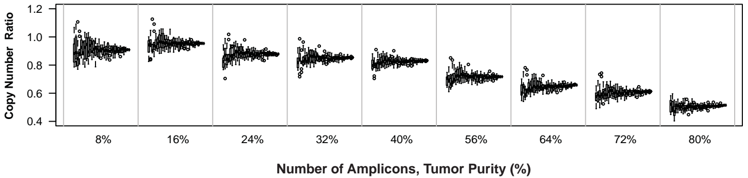
RB1 Fold Change Estimate for Increasing Number of Amplicons and Tumor Purity
