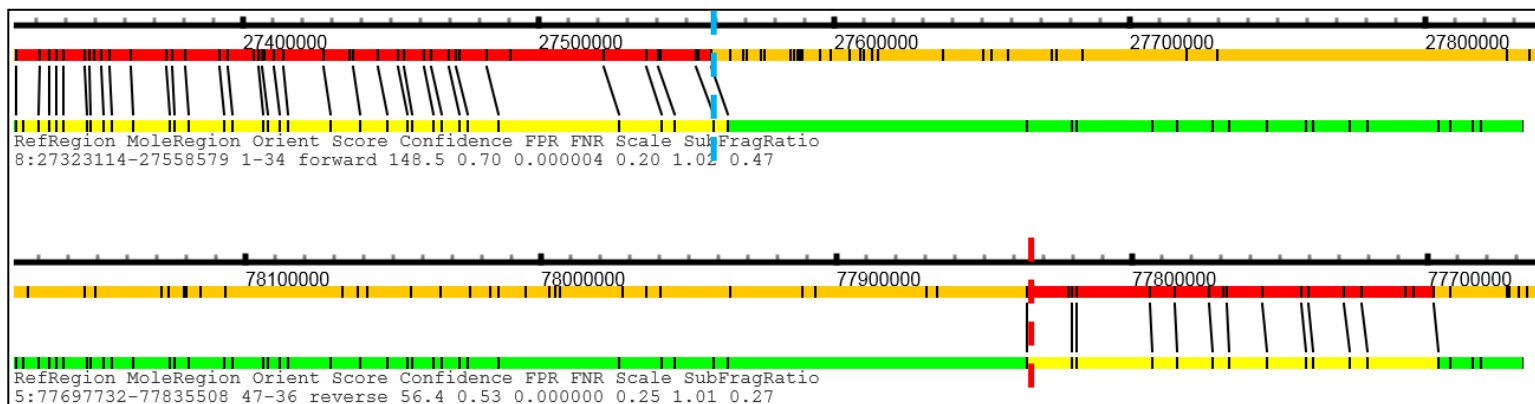
Molecule 1
