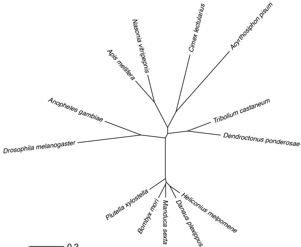
Additional File 4. Phylogenetic relationships among 13 insect taxa used for comparative genomic analysis in this study. The scale bar represents expected amino acid substitutions per site.
