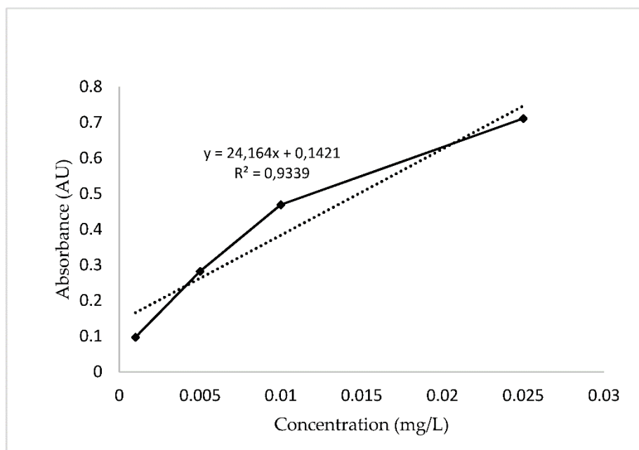
Figure S1. Standard curve for purpurin at 254 nm (- raw data; ..... linear regression)
