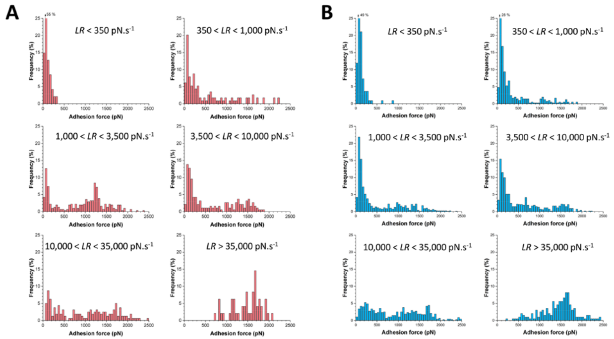
Fig. S3. The probability of forming strong bonds increases with the loading rate. (A, B) Adhesion forces were measured at various loading rates ( LR s) between AD08 cells and Lor- or L2v-tips. Small ranges of LR s were binned and the distribution of the Lor (A) and L2v (B) forces plotted as histograms (data pooled from 5 independent experiments for both Lor and L2v).
