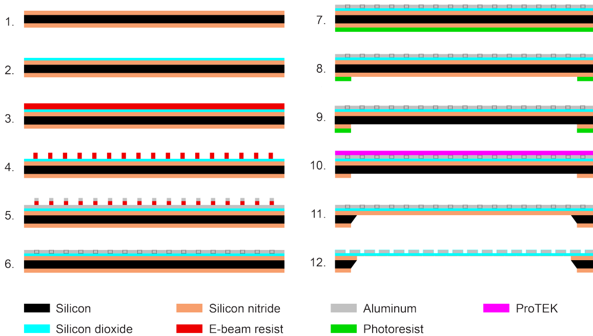
Supplementary Figure 1: Stepwise Schematic representation of NZMW fabrication process: 1. LPCVD silicon nitride coating of silicon wafer. 2. SiO 2 coating on silicon nitride on one side of wafer. 3. Spin AR-N 7520.11 negative e-beam resist. 4. Expose using EBL and develop resist. 5. Thermally evaporate 100 nm of aluminum. 6. Liftoff resist. 7. Spin S1818 positive photoresist on reverse side of the wafer. 8. Expose and develop positive photoresist. 9. Etch silicon nitride windows with reactive ion etching. 10. Spin and bake protective ProTEK on ZMW surface (on top of aluminum). 11. KOH etch silicon. 12. Remove ProTEK and deposit ALD SiO 2 .
