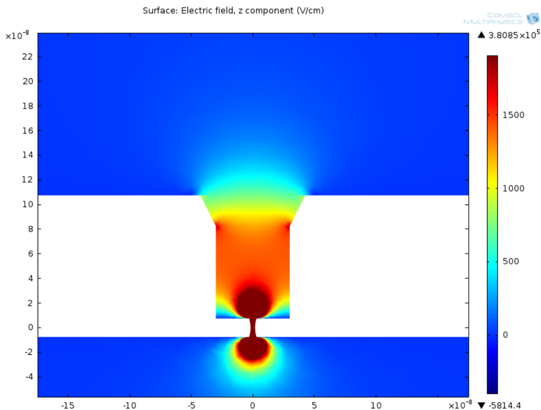
Supplementary Figure 3. The numerical solution for the DC electric field in and around a 100 nm-high ZMW with a 3 nm nanopore under 500 mV bias. To match the observed ZMW geometry, it has a 60 nm base diameter with a truncated cone structure having an 85 nm outer diameter. The electrolyte contains a 400 mM KCl concentration and the pore has a 5 nm effective height. Color scale represents the magnitude of the electric field's z component
