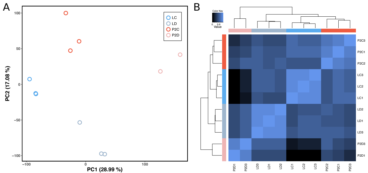
Figure S6. Replicate comparison across samples. A) Principal Component Analysis of the replicates of LC, LD, P2C and P2D based on the gene expression. B) Heatmap visualizing the sample correlation of LC, LD, P2C and P2D based on expression patterns (FDR \leq 0.05 ) by means of a Pearson correlation measure. Strong correlation is indicated by light blue while a weaker correlation is depicted by darker shades.
