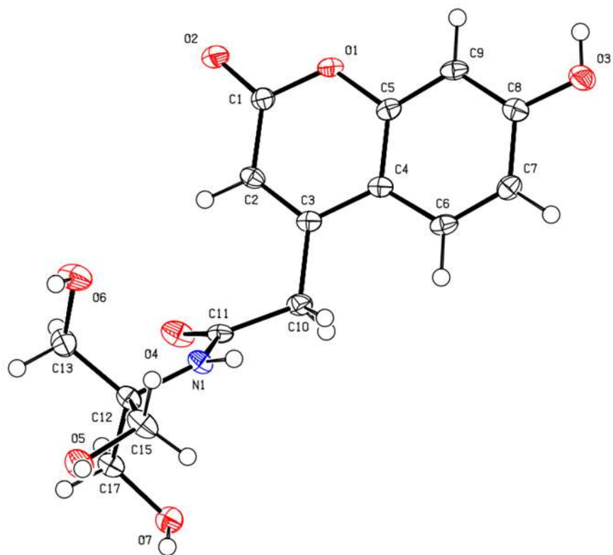
S1D Fig. Crystal structure of CT51.
