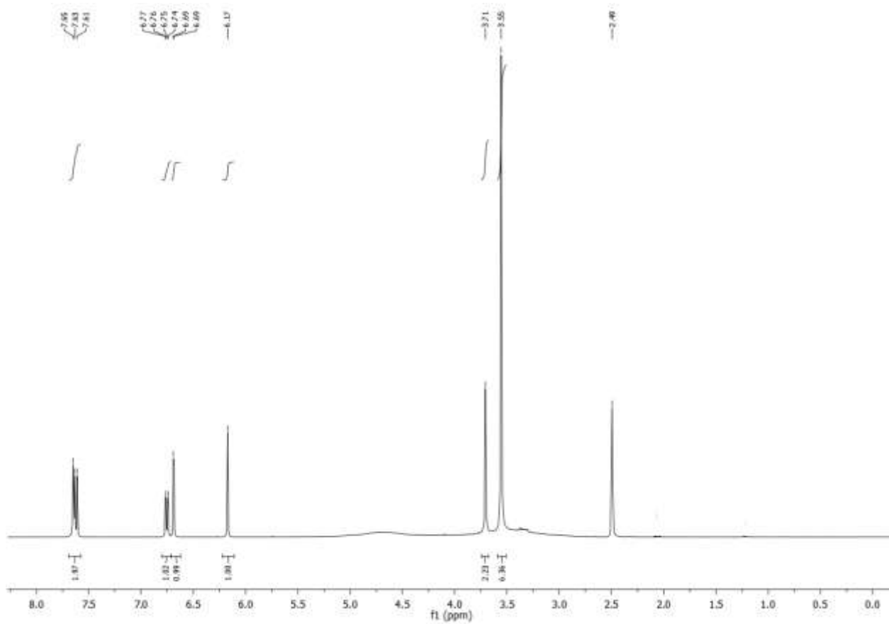
S1A Fig. Spectral properties of CT51. 1 H-NMR spectrum.
