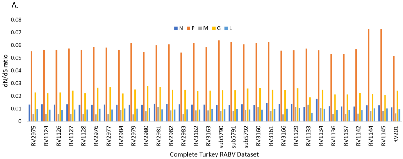
Fig S3: dN/dS ratios of consensus sequences using RV303 as reference, across all Turkey viruses ordered by collection date. (A) Individual genes, (B) average dN/dS ratios across all 5 genes. Viruses divided into following groups; pre-host shift (triangle), early phase (circle), late phase (square). Fox samples (black), dog samples (grey).
