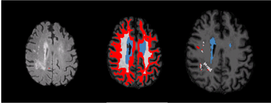
Supplemental Figure 1. Regional White Matter & Leukoaraiosis. This figure depicts a T2 FLAIR slice with white matter hyperintensities (left). A slice with a “regional mask” (middle) separated into a periventricular region (blue), deep region (white) and infracortical region (red). A slice (right) depicts the regional leukoaraiosis (LA) mask (blue = periventricular LA; white = deep LA; red = infracortical LA) defined by the intersection of leukoaraiosis mask and the regional white matter mask.
