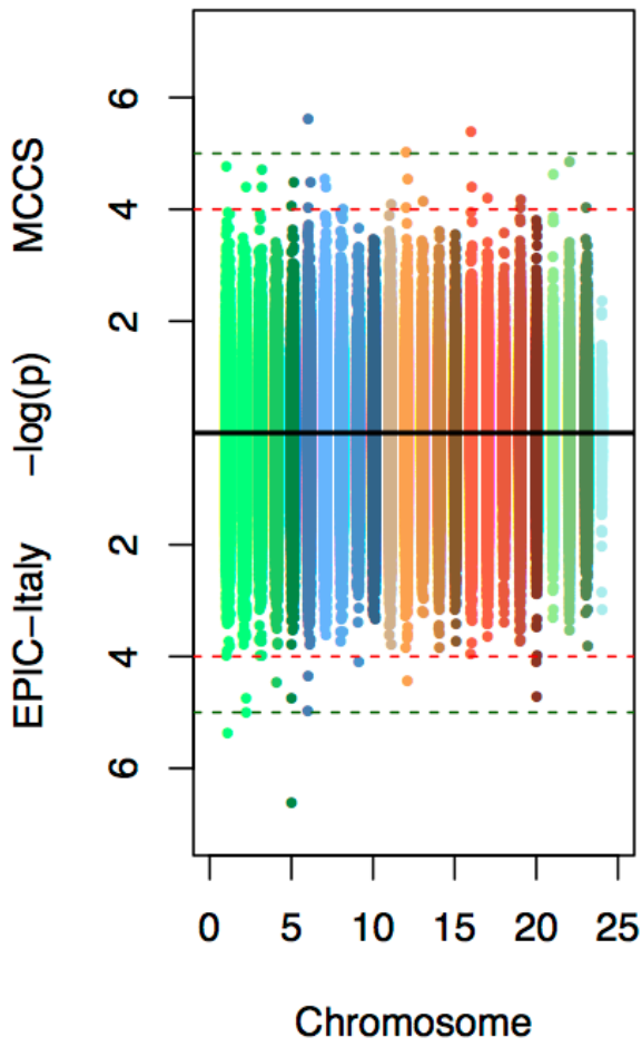
Manhattan Plot
