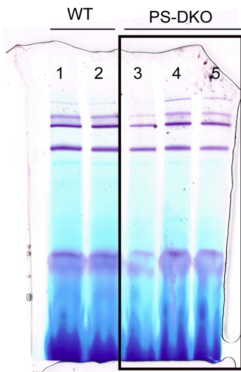
Complex I in gel activity
