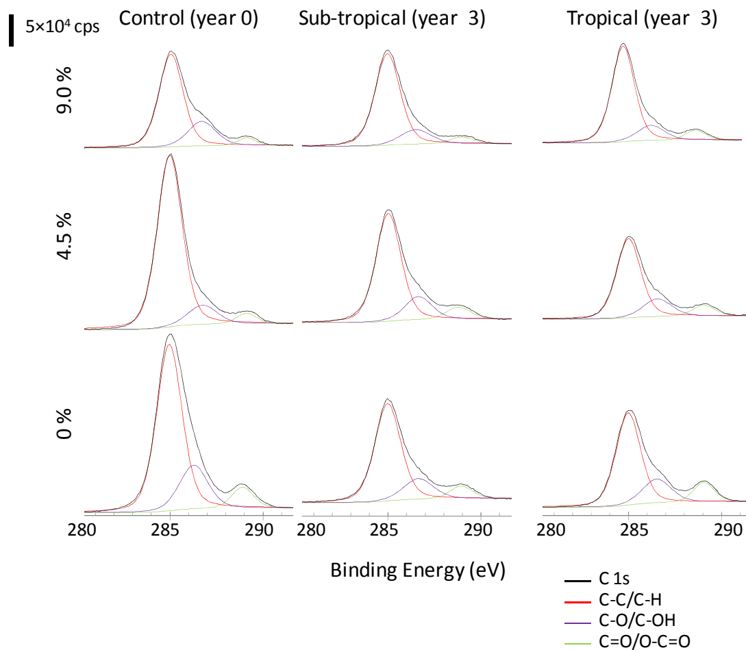
S3 Fig. Deconvolution analyses of XPS C 1s high resolution spectra of pure polyester (0% SiO 2 NPs) and polyester composite coatings (4.5% and 9% SiO 2 NPs) on steel substrata under sub-tropical and tropical climates after 3 years of environmental exposure.
