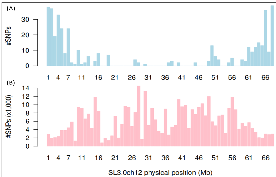
Fig S1. Physical positions of SNP markers across the tomato chromosomes (Chr00 – Chr12) except ch06 using R package. The SNP markers were generated using the next-
